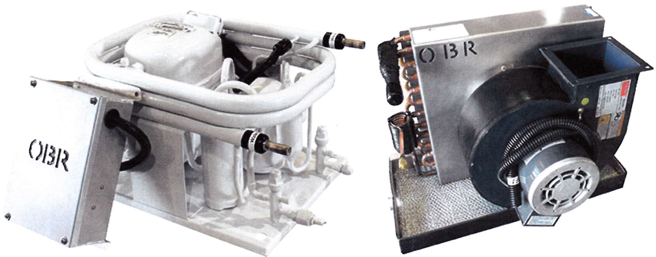
Seawater-cooled Condenser Unit and Fan Coil Unit Marine Split System Air Conditioner
