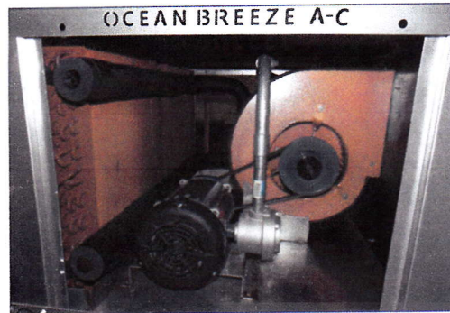
This is an example of an 6 TON (72,000 BTU) Explosion Proof Fan Coil Unit .
