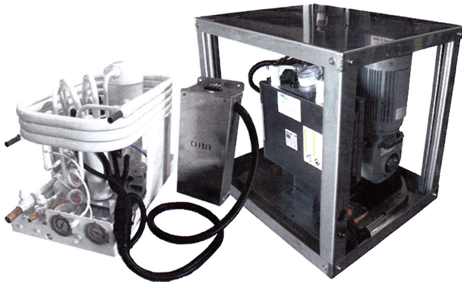
Ice Machine Split System with Water-cooled Condensing Unit
