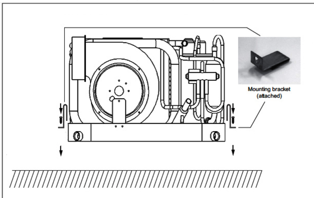
FIGURE 5. Mounting brackets installation overview
